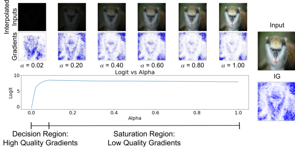
Figure 2: The figure illustrates the IG attribution method and saturation effects within path integrals. The top row shows interpolated inputs and the second row shows the corresponding gradients. The IG attribution map (shown to the right) is the average of the gradients. The third row shows the logit- \alpha curve, which defines the decision and saturation regions. It can be observed that the gradients from the decision region are of higher quality than the saturation region.
