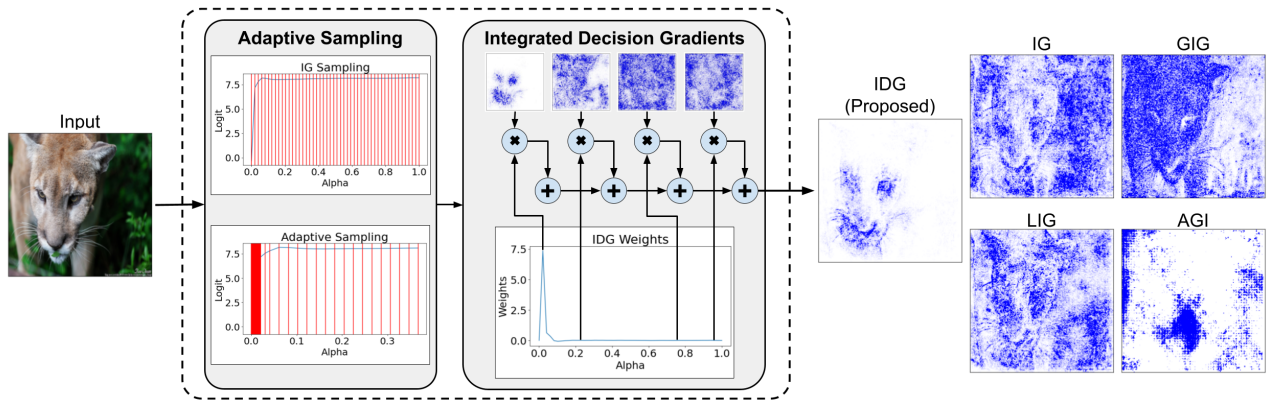
Figure 1: (left) An overview of the adaptive sampling algorithm, and the IDG attribution method. (right) A preliminary visual comparison of IDG with IG (Sundararajan, Taly, and Yan 2017), LIG (Miglani et al. 2020a), GIG (Kapishnikov et al. 2021b), and AGI (Pan, Li, and Zhu 2021b).
