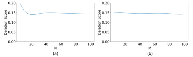
Figure 7: The change in the deletion score of IDG with AS averaged over 10 images by varying (a) N and (b) M . In the graphs, N ( M ) is varied from 5 to 100 while M ( N ) is set to 50. It is seen that the most stable scores are located where N = M .
