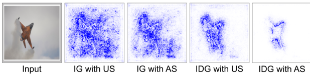
Figure 8: Given the input, attributions created by IG using uniform sampling (US) and AS are compared to attributions created by IDG with US and AS. Since AS applied to IG does not meaningfully improve performance over IG with US, and IDG with US provides a higher quality attribution, we determine that IDG, not AS, is the solution to the saturation problem. This is further exemplified by the improvement seen in IDG with AS, reinforcing the idea that AS gives IDG access to better gradients, but IDG is the solution to the saturation problem.
