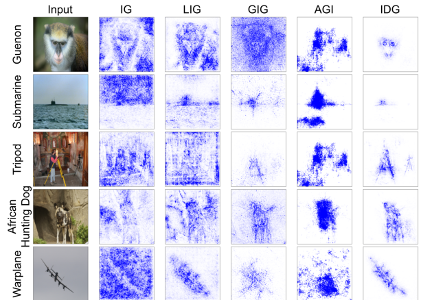
Figure 6: Qualitative comparison of attributions computed using the IG (Sundararajan, Taly, and Yan 2017), LIG (Miglani et al. 2020a), GIG (Kapishnikov et al. 2021b), and AGI (Pan, Li, and Zhu 2021b), and IDG methods. It is seen in the selected examples that IDG solves the saturation problem and outperforms the state-of-the-art path-based attribution methods in visual quality.
