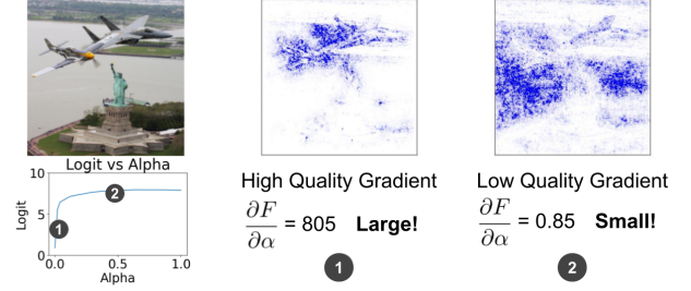
Figure 3: An illustration of the relationship between importance factor magnitude and gradient quality. Higher importance factors are directly related to higher quality gradients.
